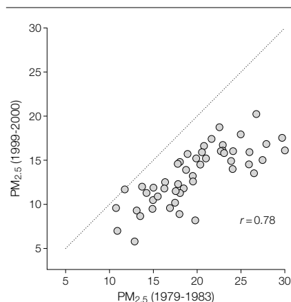
Figure 1. Mean Fine Particles Measuring Less Than 2.5 \mu\text{m} in Diameter (PM 2.5 )
